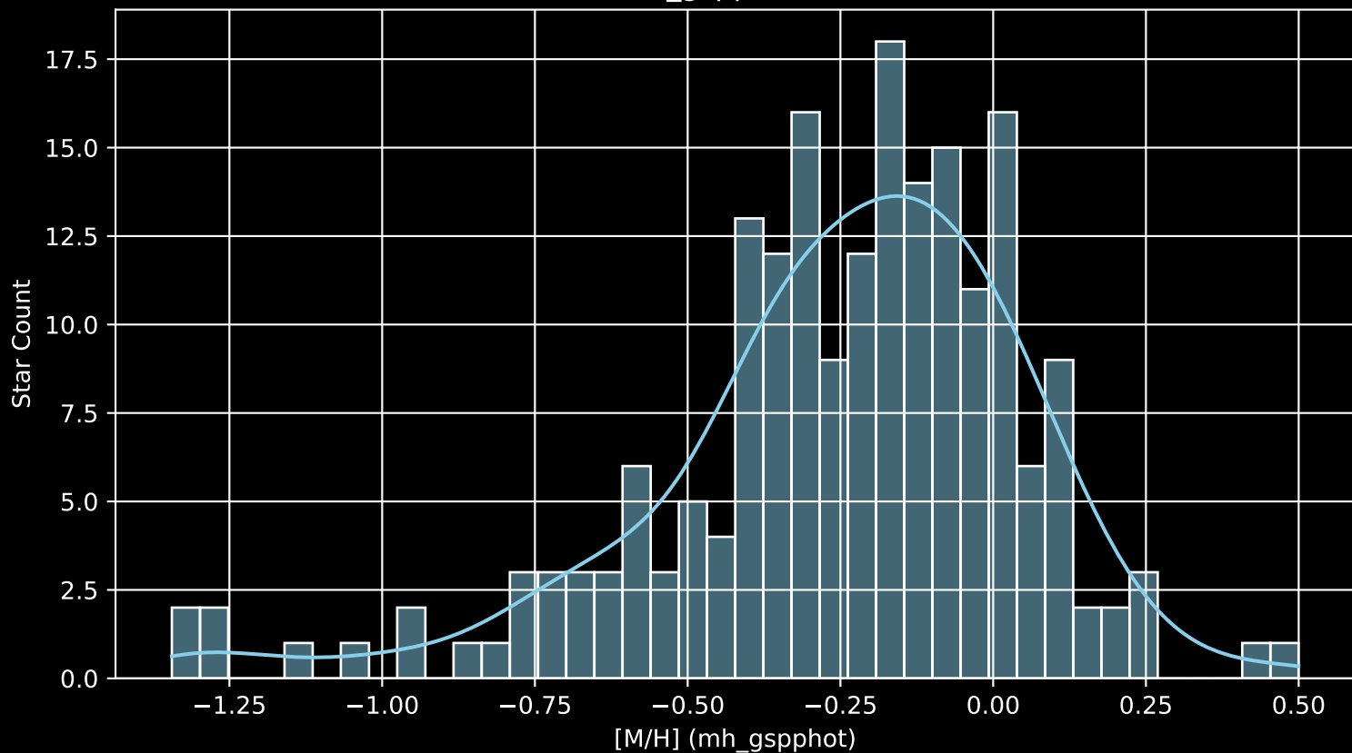
APOGEE DR17 Field: [090-30 [M/H] (mh_gspphot) (n= 200)
