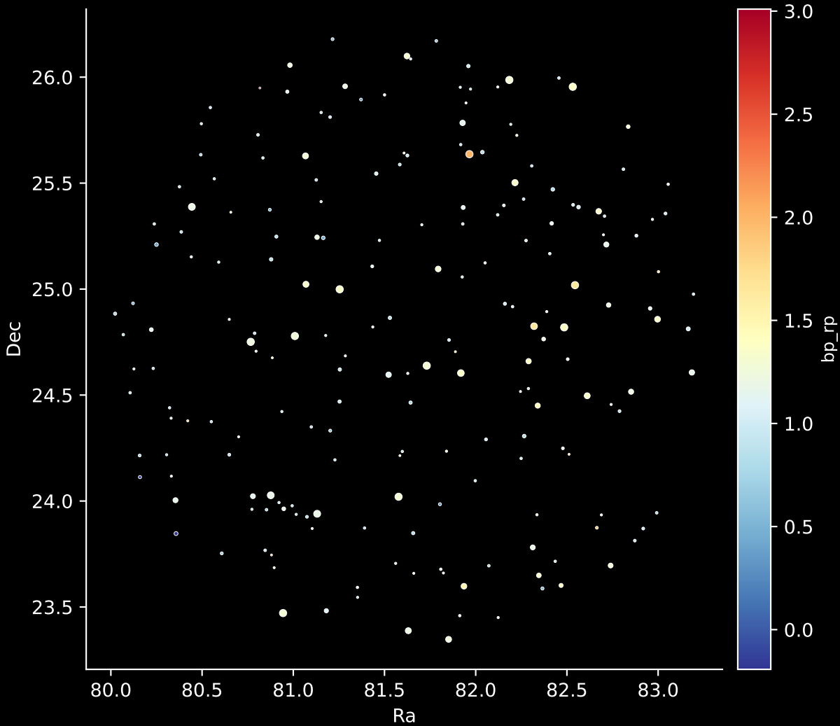
APOGEE DR17 Field: [090-30] Stars: 202
