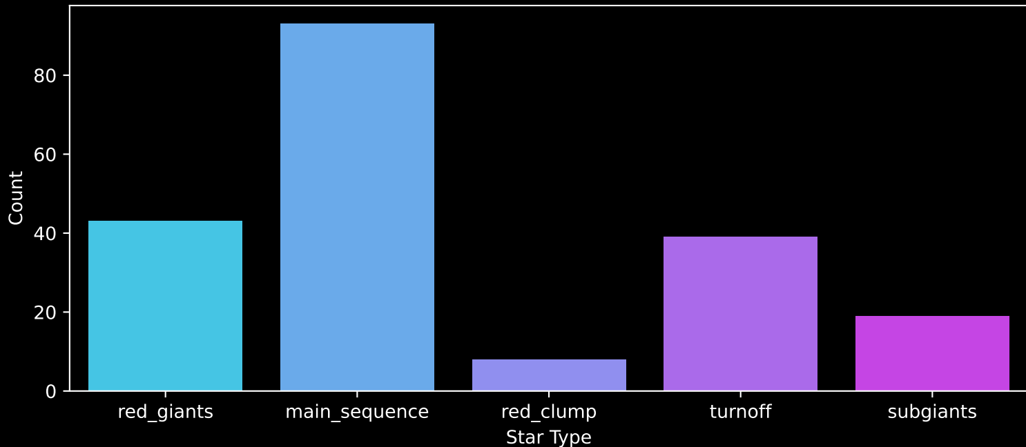
APOGEE DR17 Field: [090-30] Count plot of Star Type
