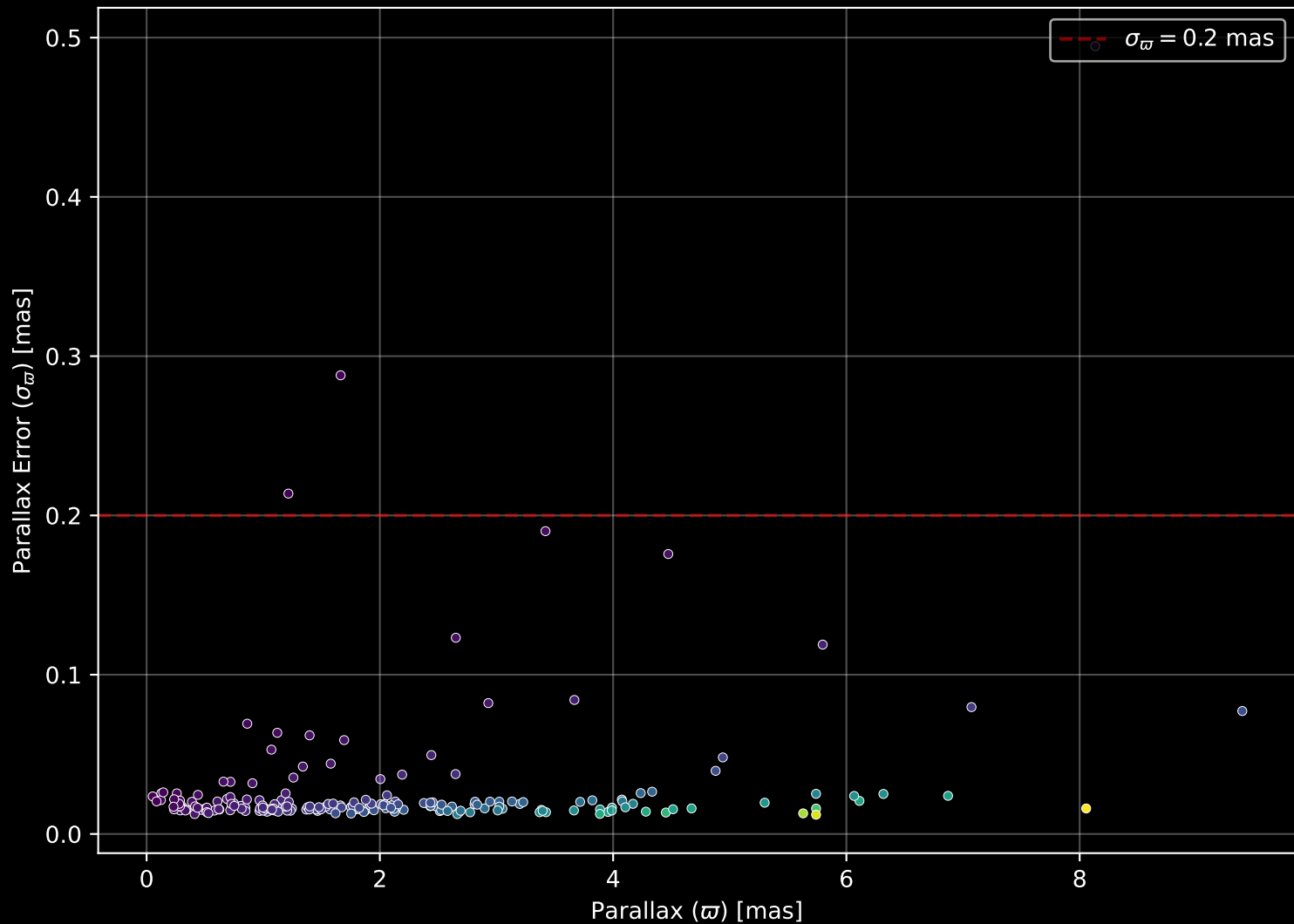
APOGEE DR17 Field: [090-30] Parallax Quality (n= 202)
