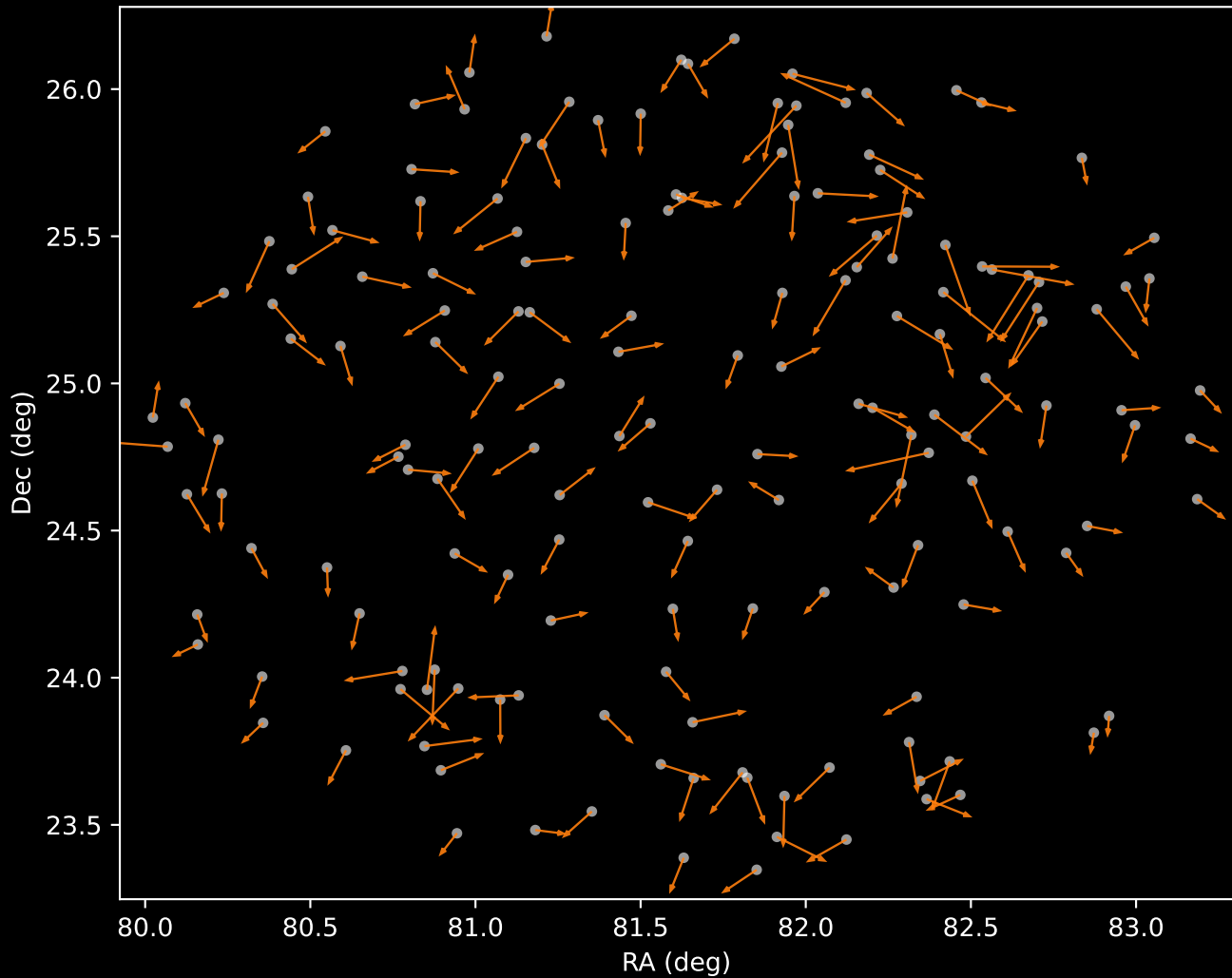
APOGEE DR17 Cluster 2 Proper Motion Vectors (n=165)
