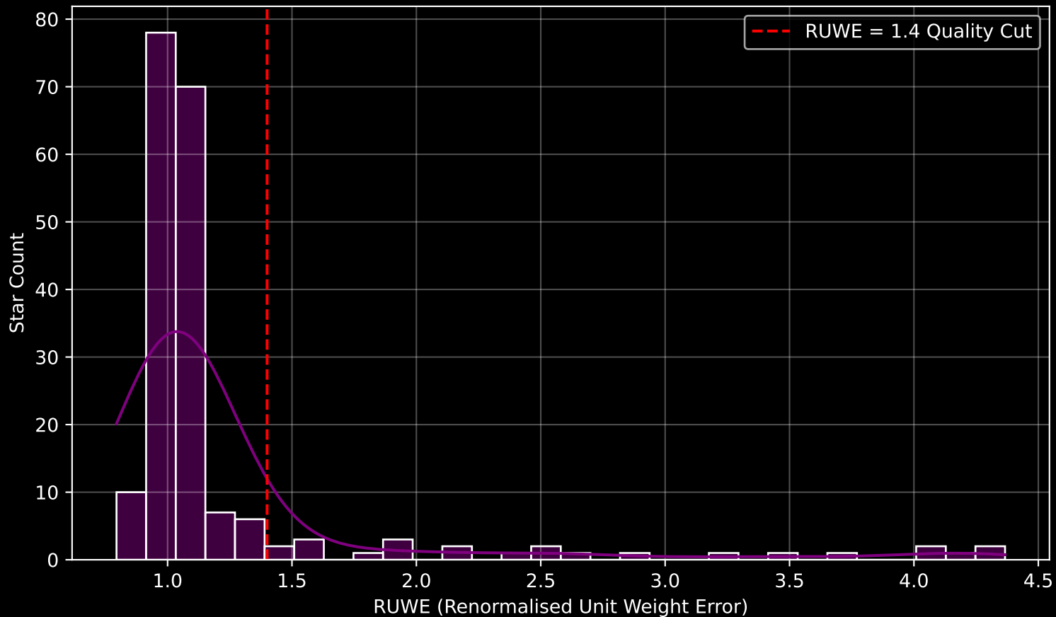
GAPOGEE DR17 Field [090-30] RUWE Distribution (n= 195)
