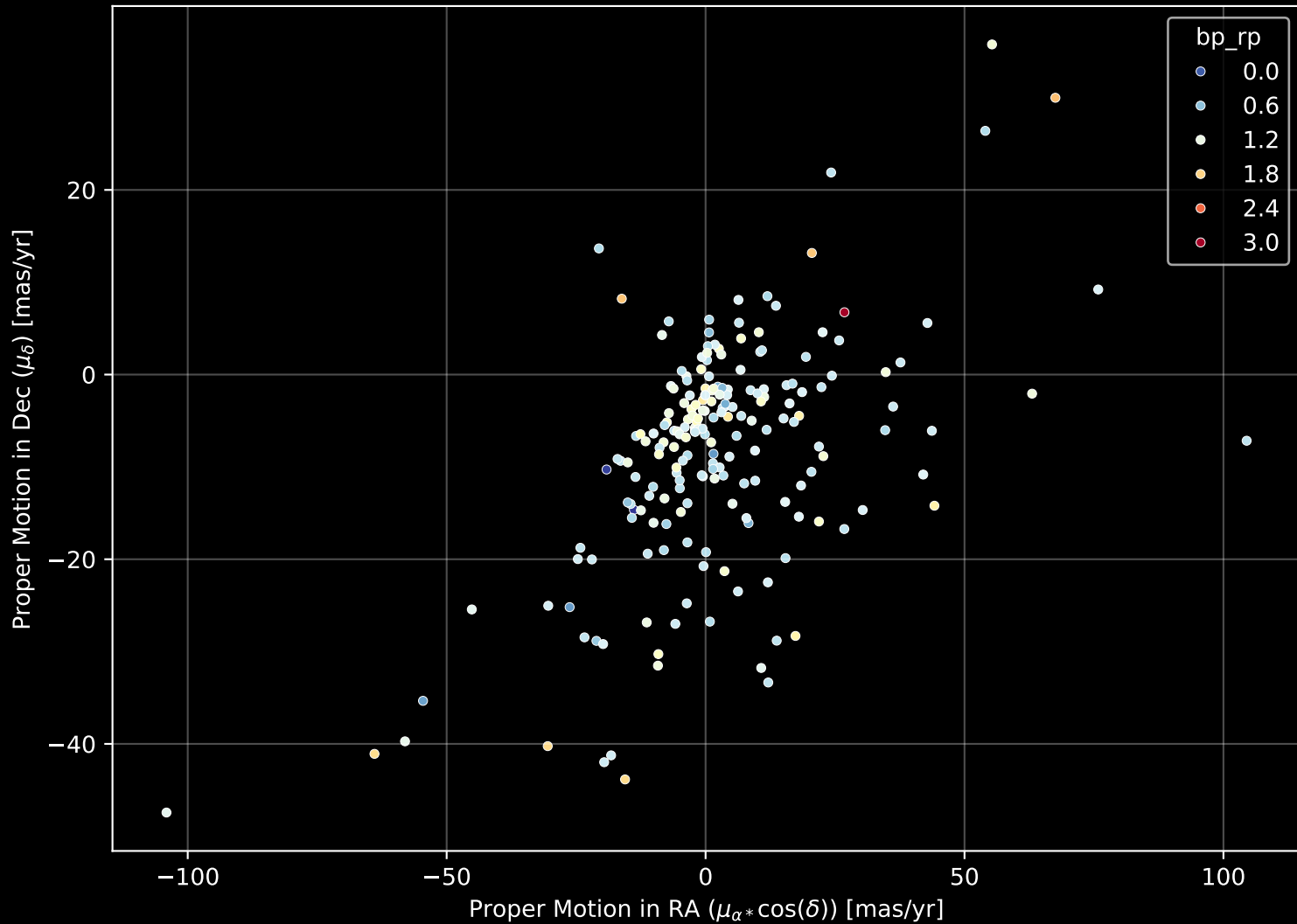
APOGEE DR17 Field: [090-30] Proper Motion Diagram (n= 202)
